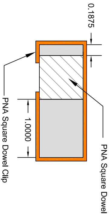
A PNA Square Dowel w/ Clip for Post Tensioned Slabs
