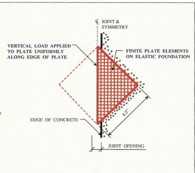
Fig. 4 - Computer model for diamond plate dowel.
