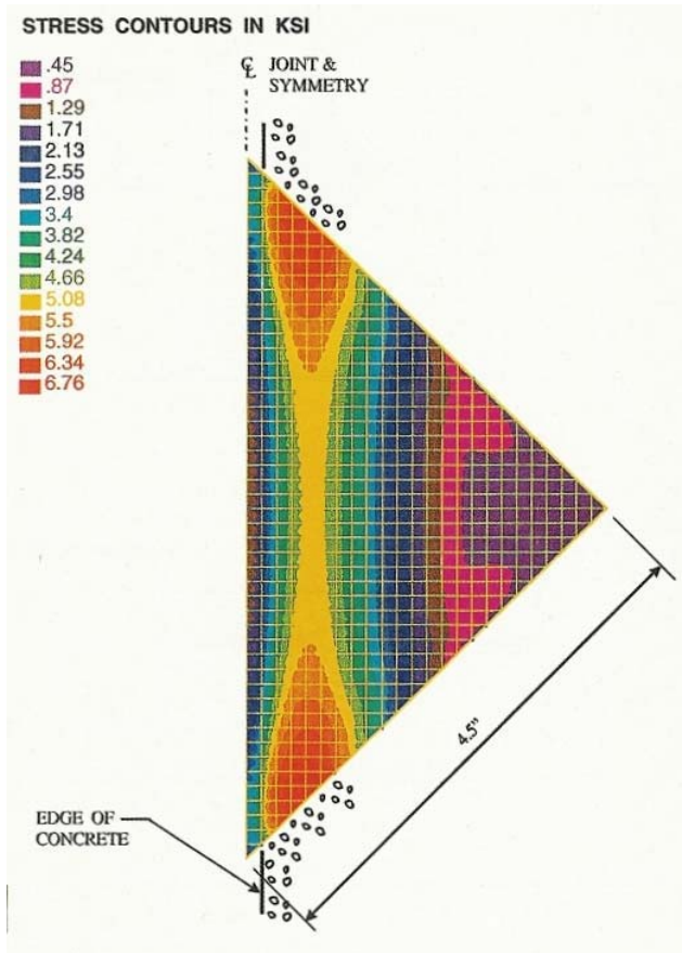
Fig. 5 - Flexural stresses for a 1/4 in. thick diamond plate dowel with a one kip load applied to the edge.
