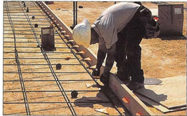
Worker installing diamond plate dowel pocket formers on base supports, which were previously attached to form. Note no form penetrations are required. Note short dowel length and long spacing as compared to typical dowels.
