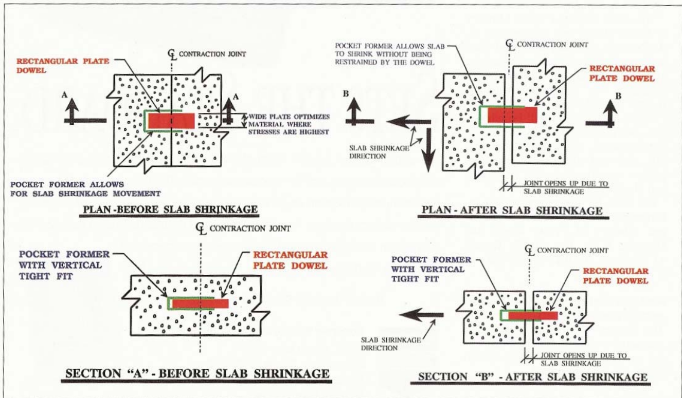
Fig. 1(a) - Rectangular plate dowel before slab shrinkage.
