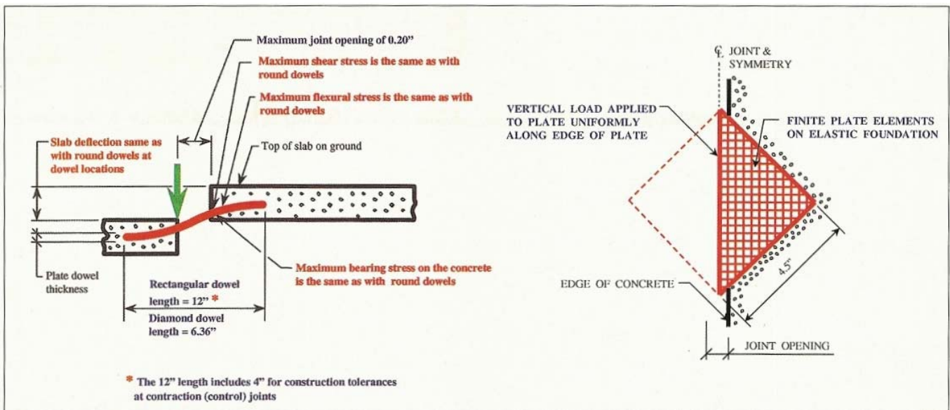
Fig. 3 - Plate dowel performance requirements.
