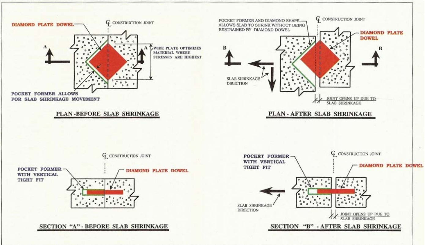
Fig. 2(a) - Diamond plate dowel before slab shrinkage.
